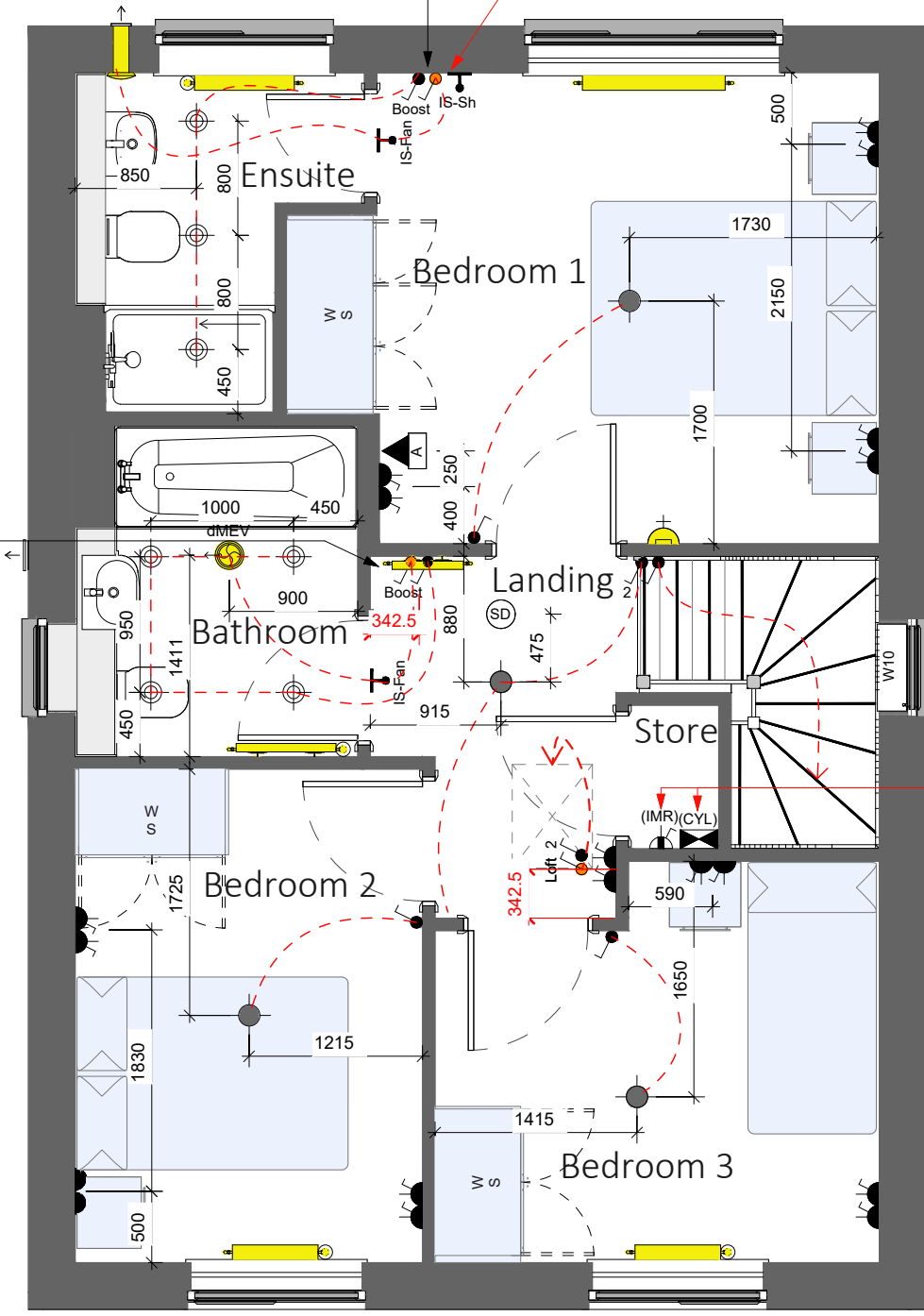
1 First Floor Electrical GA 1 : 50
