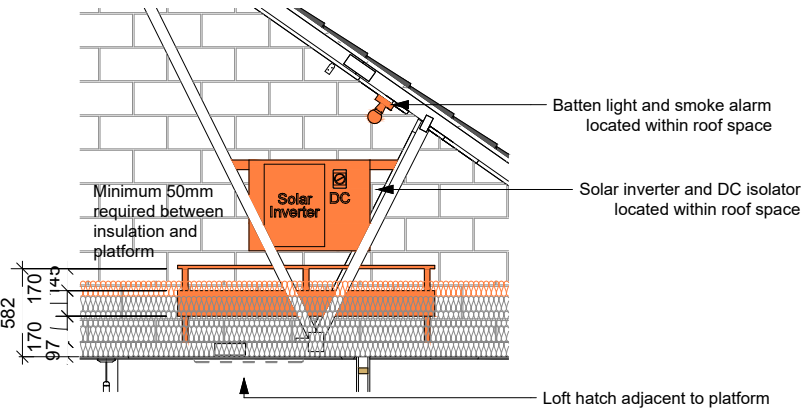
3 Solar Invertor in Loft Space (2021 Only) 1 : 50
